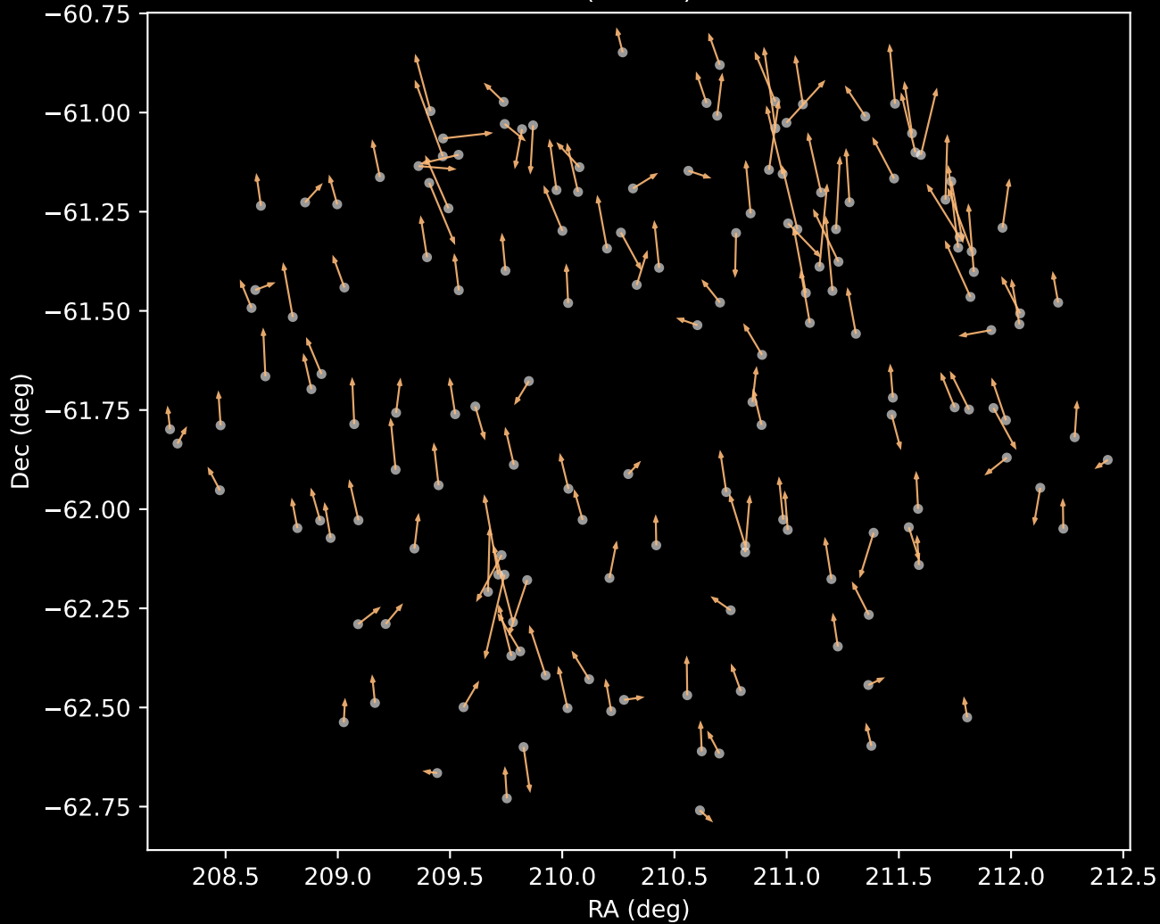
GALAH DR4 Cluster 3 Proper Motion Vectors (n=157)
