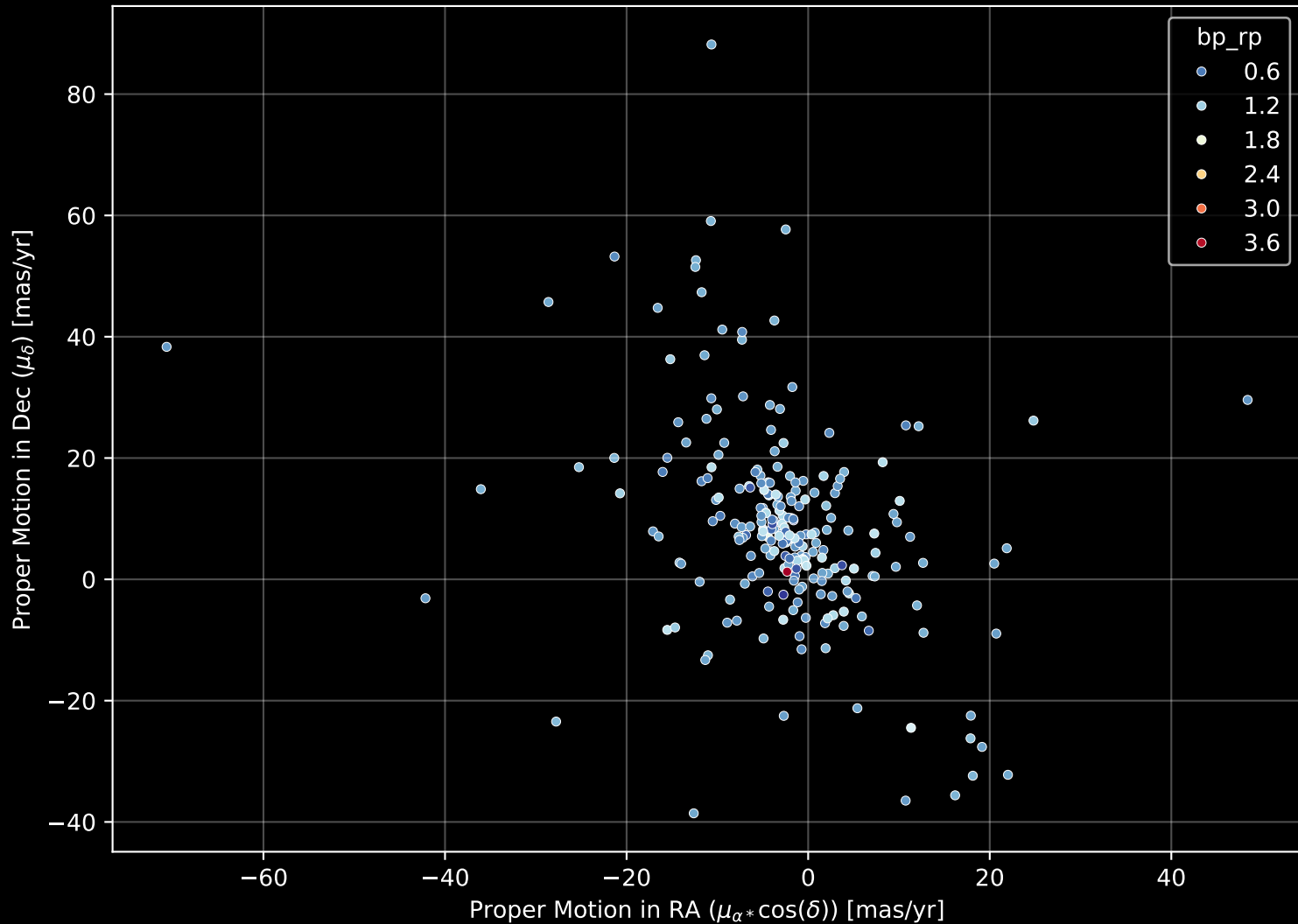
GALAH DR4 Field: [7193] Proper Motion Diagram (n= 234)
