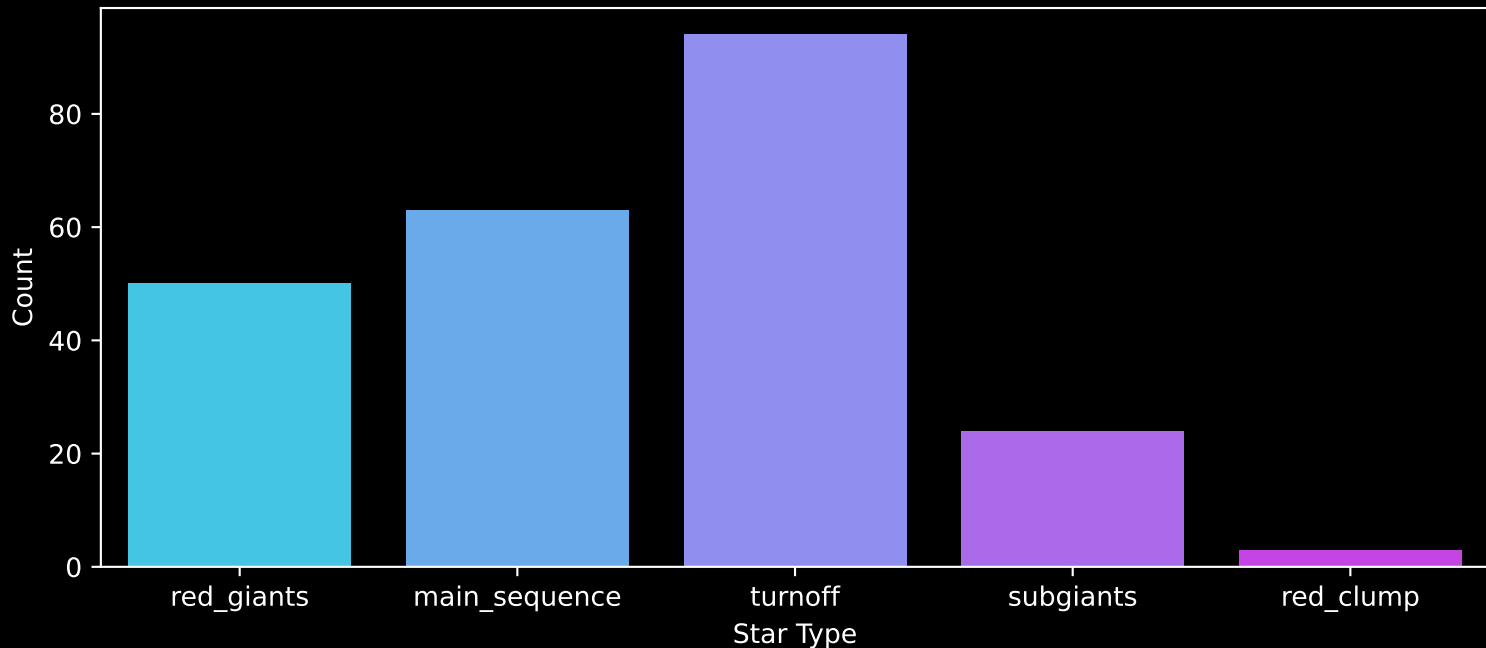
GALAH DR4 Field: [7193] Count plot of Star Type
