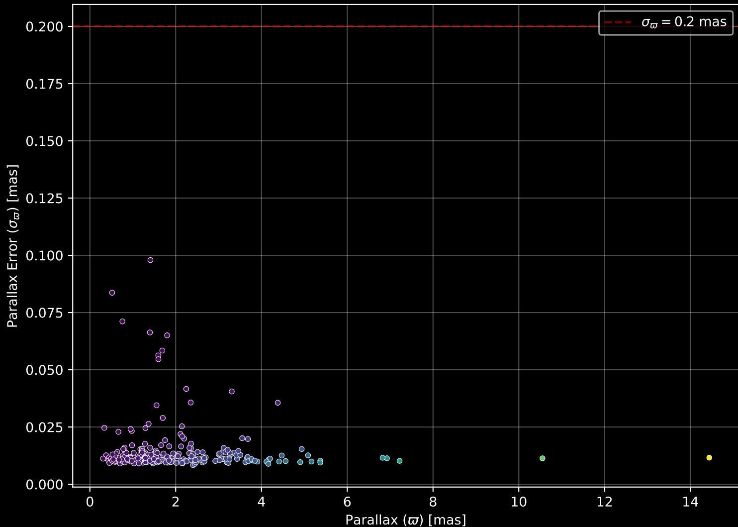
GALAH DR4 Field: [7193] Parallax Quality (n= 234)
