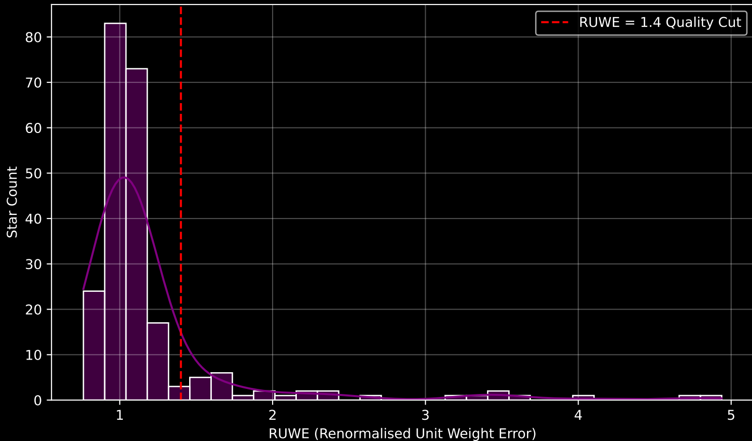
GALAH DR4 Field [7193] RUWE Distribution (n= 228)
