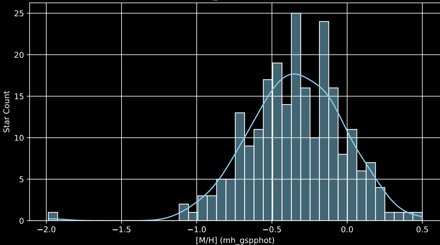
GALAH DR4 Field: [7193] [M/H] (mh_gspphot) (n= 234)
